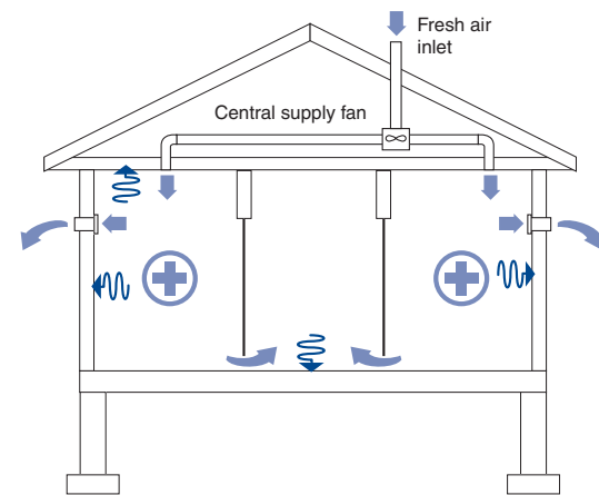
Supply ventilation
