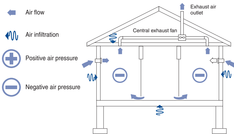
Exhaust ventilation
